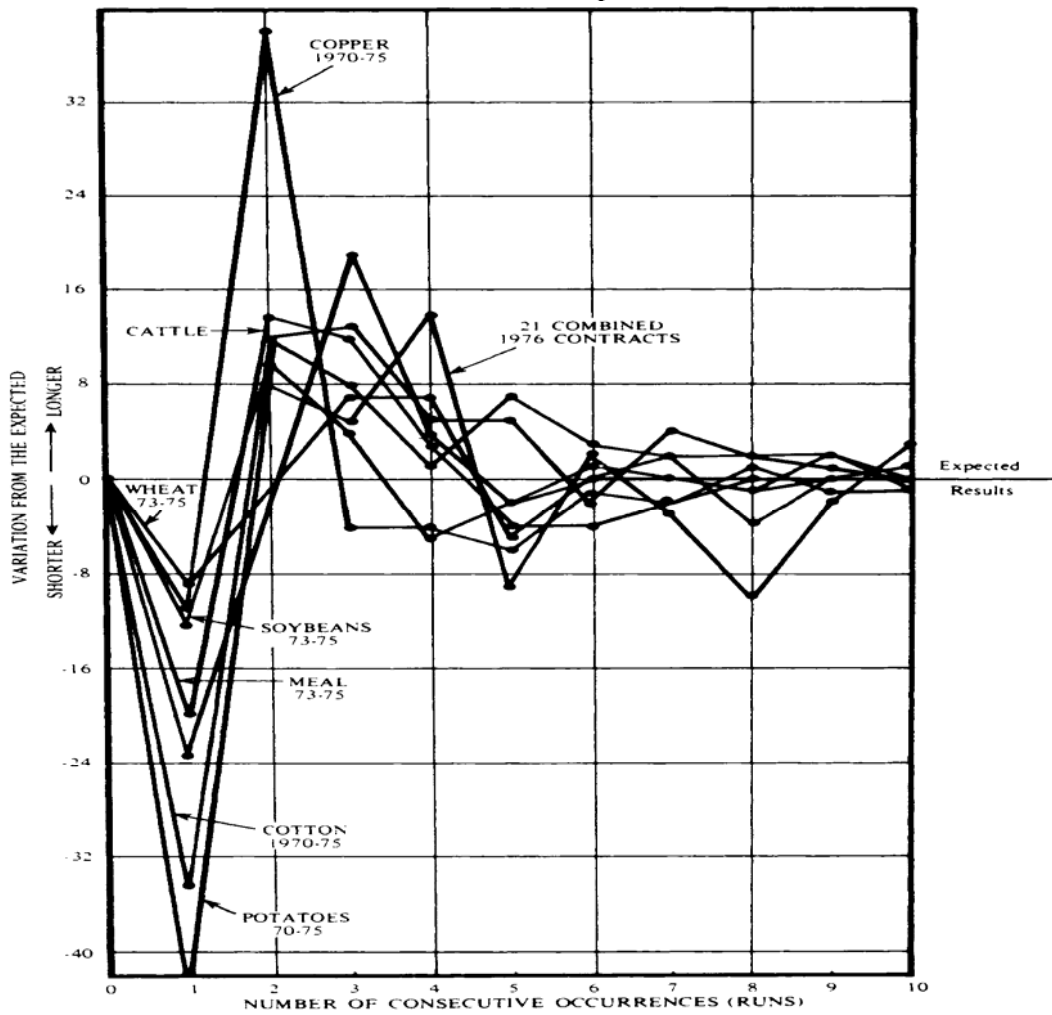
FIGURE 22-6 Actual futures movement compared with random movement.
