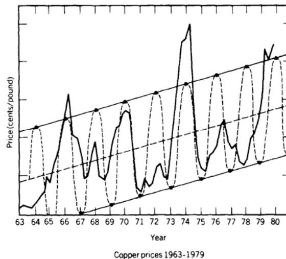
FIGURE 8-8 Copper prices 1963-1979: single-frequency copper cycle manually scaled to approximate amplitude.
