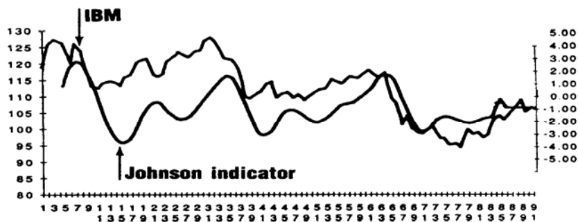
FIGURE 8-4 A triangular MACD shows an apparent cycle in IBM. Johnson indicator on IBM 2/1/88-3/30/90, IBM 2/1/88-3/30/90
