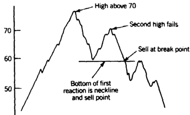
FIGURE 6-6 RSI top formation.
