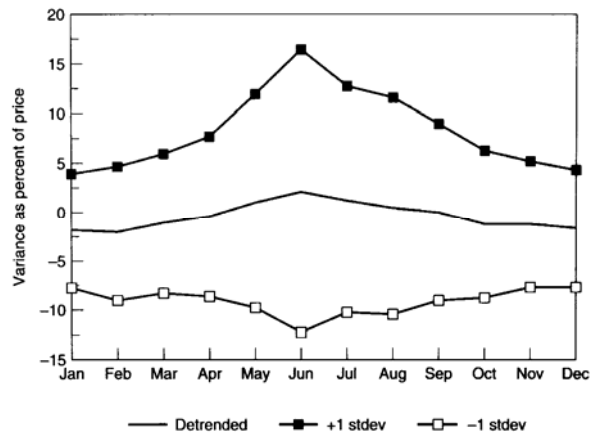
FIGURE 7-5 Soybean monthly price variation.
