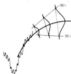
FIGURE3-10 ARIMA forecast becomes less accurate as it is used farther ahead.
