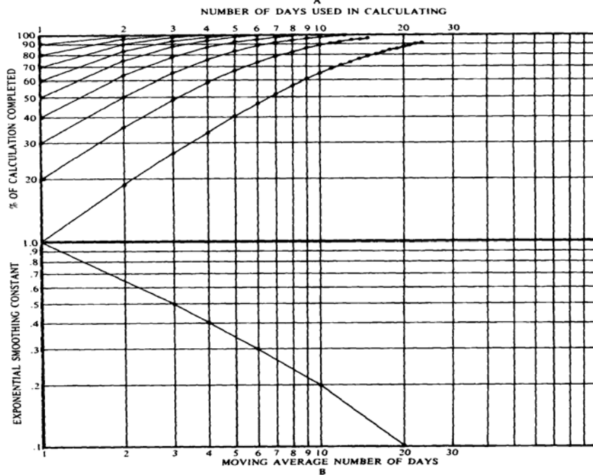
FIGURE 4-7 Evaluation of exponential smoothing.
