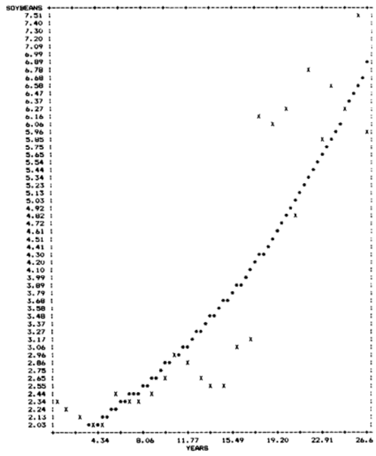
Plot of Regression Analysis
