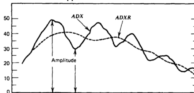
FIGURE23-9 Appearance of the ADX and ADXR.
