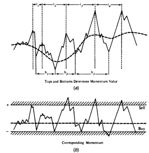
FIGURE 6-5 Relationship of momentum to prices. (a) Tops and bottoms determine momentum value. (b) Corresponding momentum.
