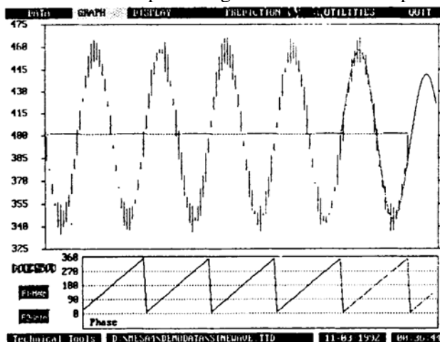
FIGURE 8-13 The phase angle forms a sawtooth pattern.
