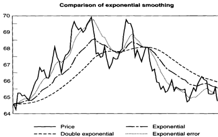
FIGURE 4-4 Comparison of exponential smoothing techniques. A simple .10 smoothing (Exp) is compared with a double-smoothed series (Dbl Exp), which applies the smoothing constant .10 first to prices, then to the smoothed series, and also to a smoothed series with the error restored (Exp Err).
