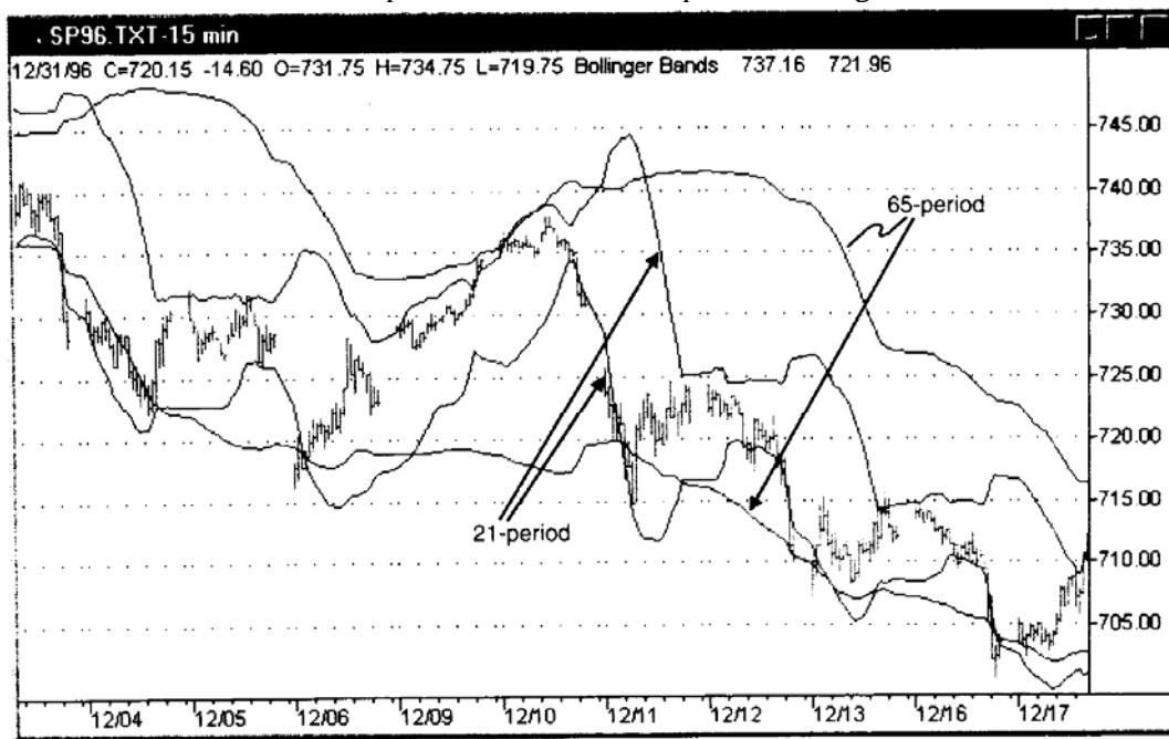
FIGURE 18-1 Comparison of 21 - and 65-period Bollinger bands.
