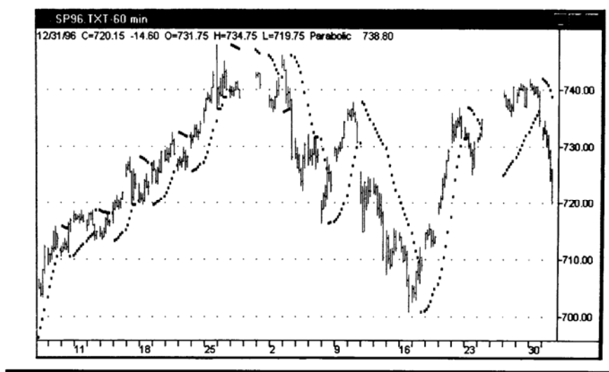
FIGURE 17-2 Parabolic Time/Price System, Feb 96 S&P 500, 60-minute chart.
