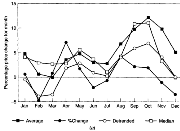
Heating oil seasonality 1980-Mar 1994 All years from continuous data
