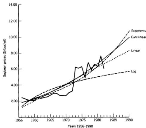
FIGURE 3-8 Least-squares approximation for soybeans using linear, curvilinear, logarithmic, and exponential models.
