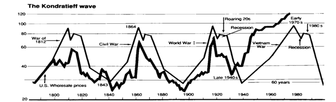
FIGURE 8-3 The Kondratieff Wave.
