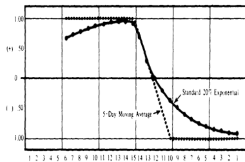
FIGURE 4-6 Comparative changes in straight and exponential moving averages.
