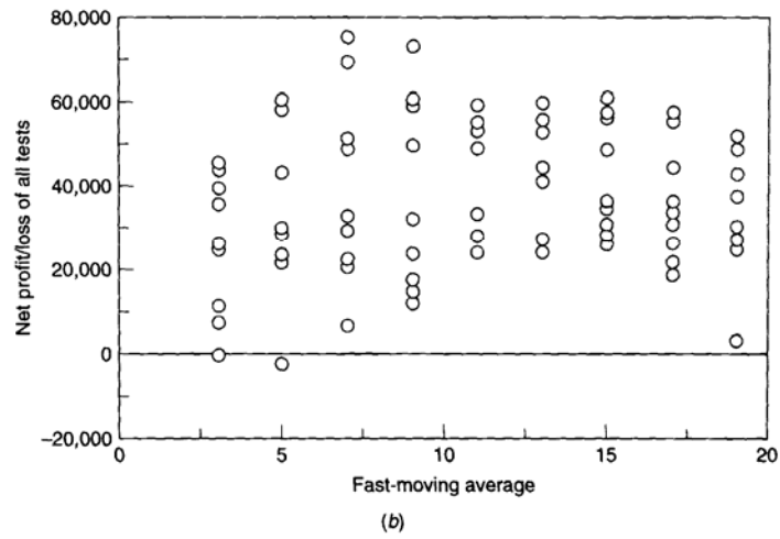
Alternate display of 2-parameter test IMM Swiss franc 1986-1996
