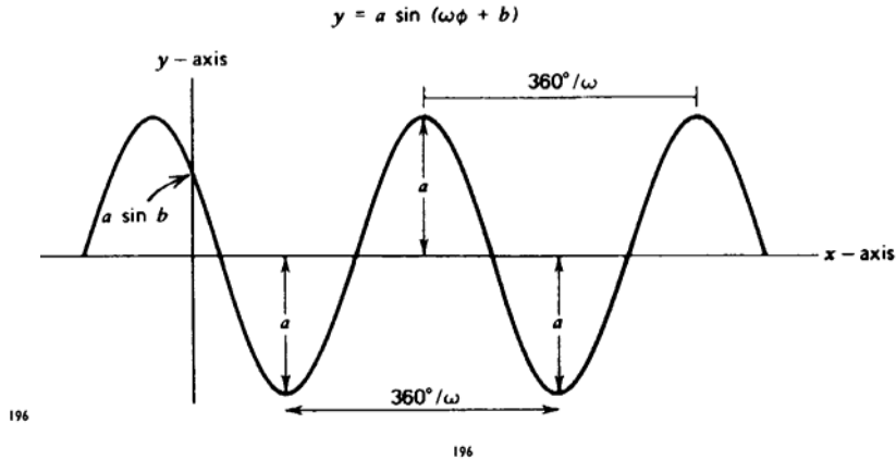
FIGURE 8-5 Sinusoidal wave.
