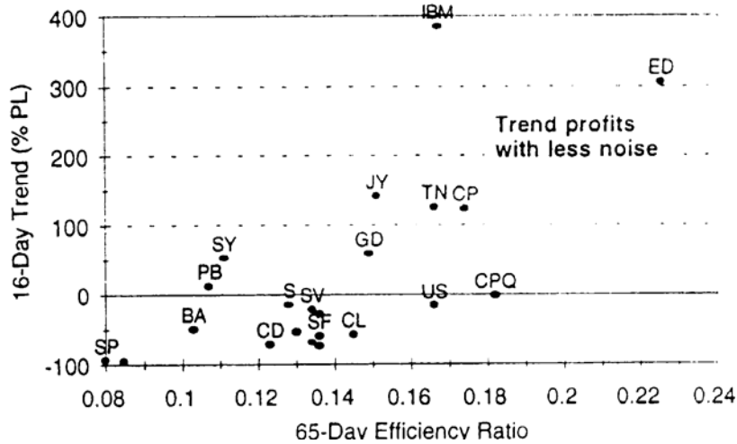
(65-Day Eff Ratio and 16-Day Trend)
