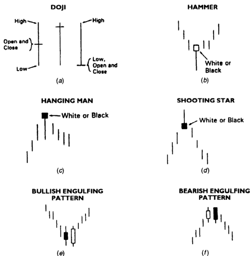
FIGURE9-10 Popular candle formations.
