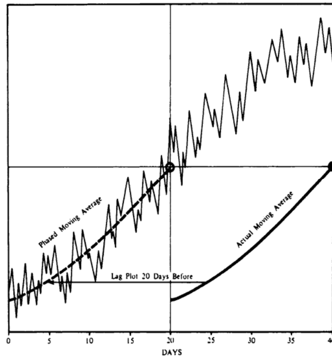
FIGURE 8-14 Phasing.
