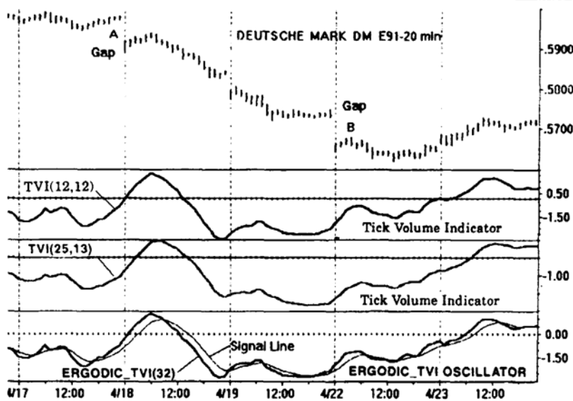
FIGURE 10-1 Blaus Tick Volume Indicator.
