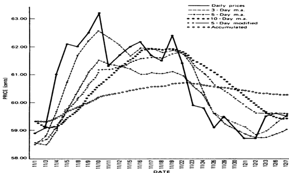
FIGURE 4-1 A comparison of moving averages.
