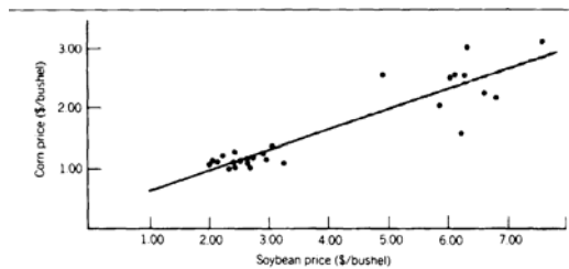
FIGURE 3-3 Scatter diagram of corn, soybean pairs with linear regression solution.
