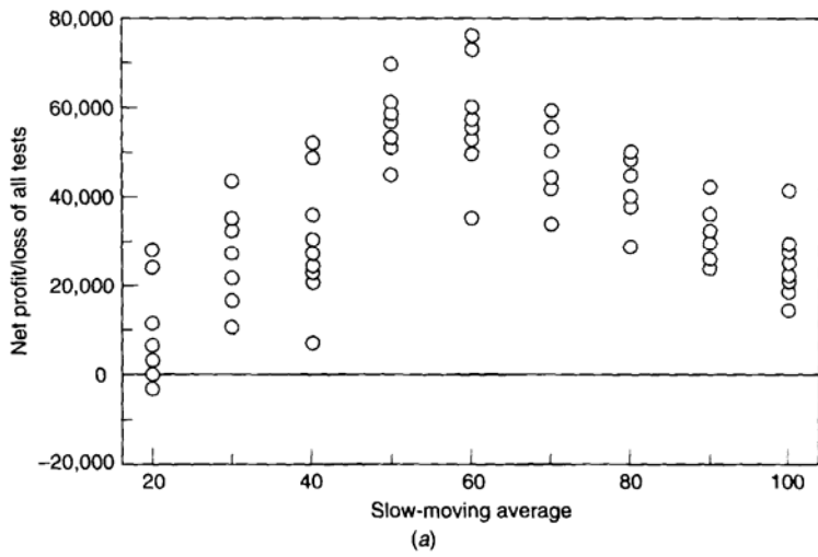
Alternate display of 2-parameter test Swiss franc 1986-1996
