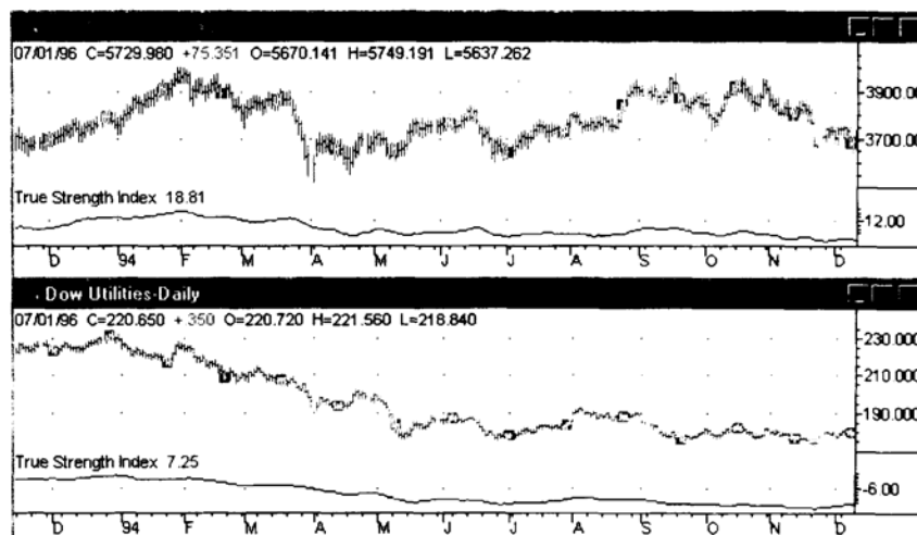
FIGURE 6-15 Double-smoothed momentum applied to the Dow Jones Average and Dow Jones Utilities, showing divergence .
