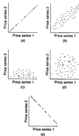
FIGURE 3-4 Degrees of correlation. (a) Perfect positive linear correlation ( r^2 = 1 ). (b) Somewhat positive linear correlation ( r^2 = .5 ). (c) and (d) No correlation ( r^2 = 0 ). (e) Perfect negative linear correlation ( r^2 = -1 ).
