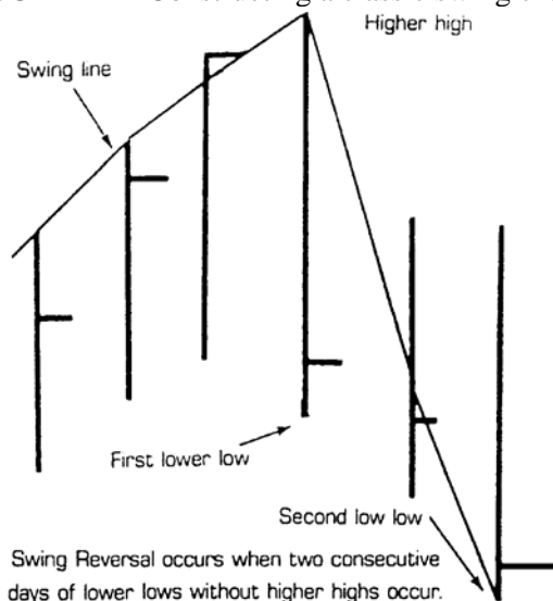
FIGURE 12-2 Constructing a classic swing chart.
