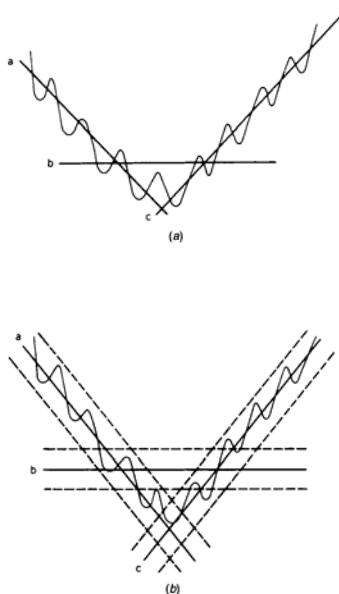
FIGURE 3-11 Linear regression model. (a) Simple penetration of the regression lines. (b) Penetration of the channel formed by confidence bands .
