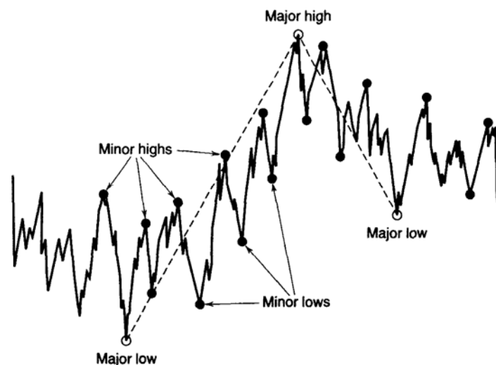
FIGURE 12-7 Major and minor swings.
