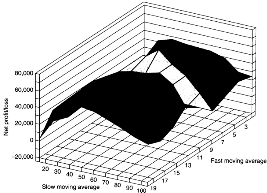
IMM Swiss franc, 1986-1996
