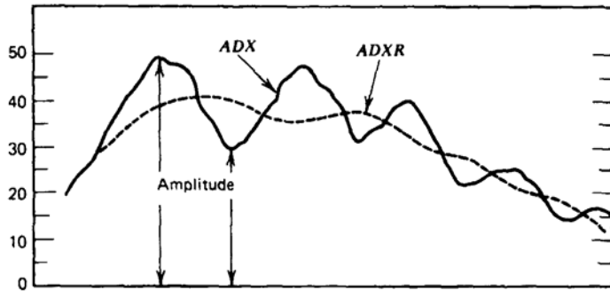
FIGURE23-9 Appearance of the ADX and ADXR.
