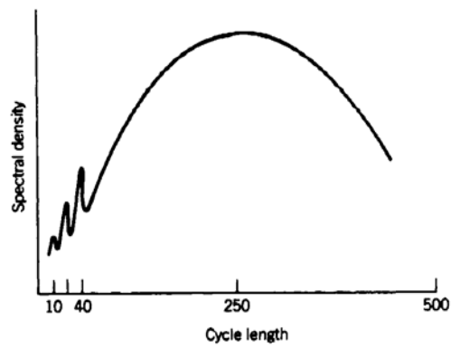
FIGURE 8-11 10-, 20-, and 40-day cycles, within a 250-day seasonal.
