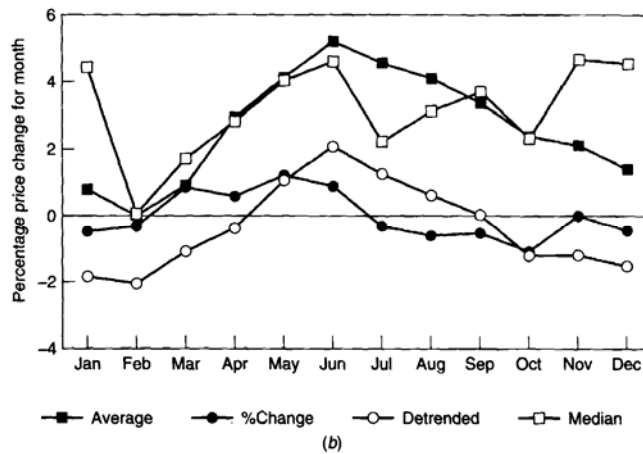
Soybean seasonality 1969-1993 All years from continuous data
