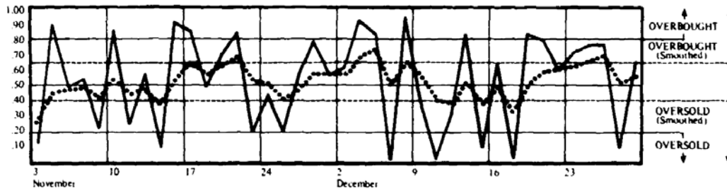
FIGURE 6-10 A/D Oscillator
