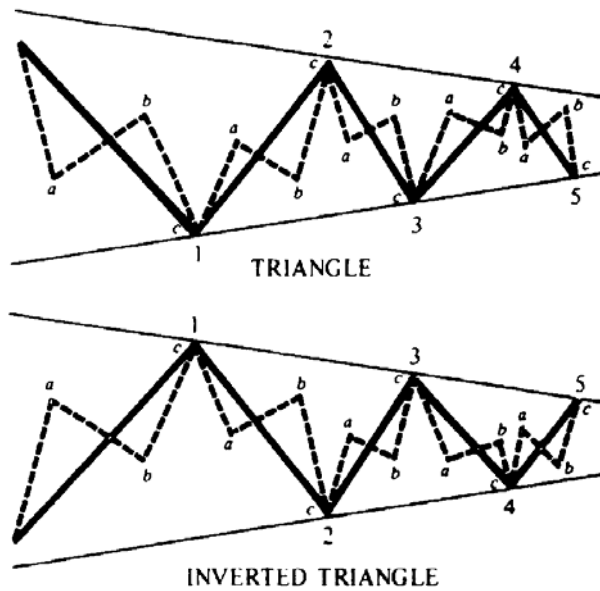
FIGURE 14- 10 Compound correction waves.
