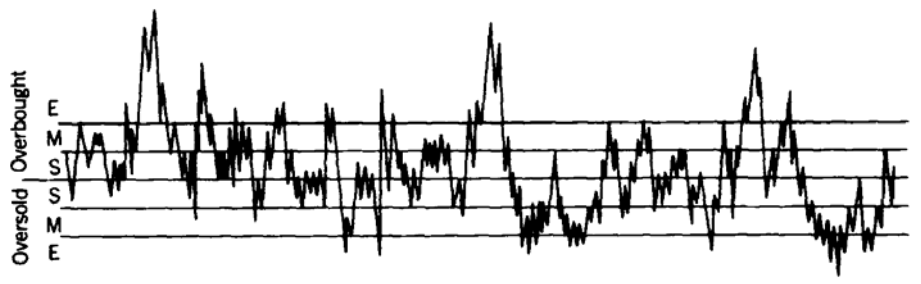
FIGURE 22-8 Countertrend alternatives using detrended price series.
