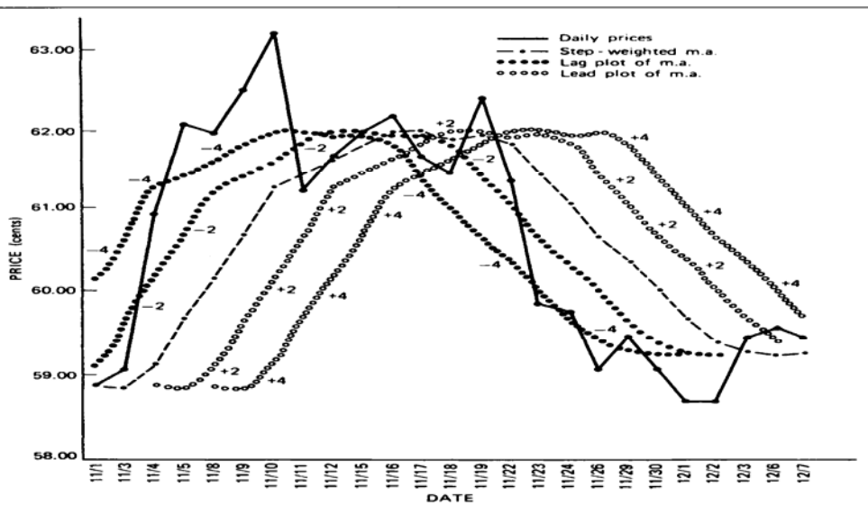
FIGURE 4.2 Plotting lag and lead for a 10-day step-weighted moving average with weighting factors of 10, 9, 8, . . .
