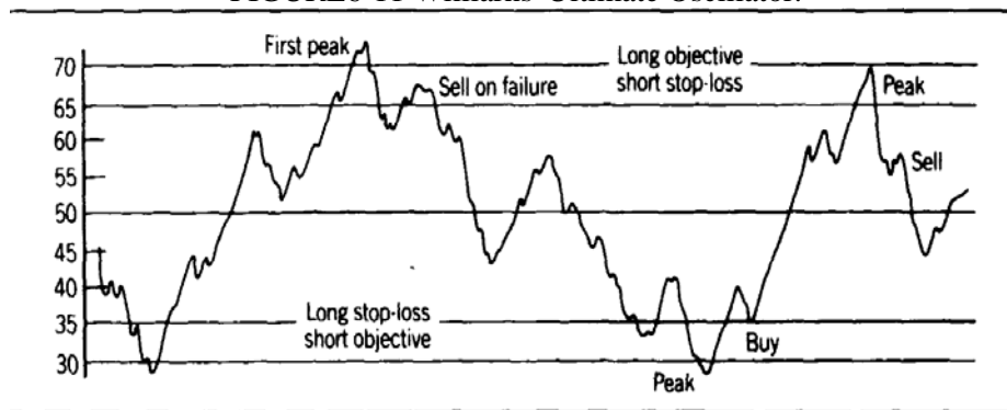
FIGURE6-11 Williams' Ultimate Oscillator.
