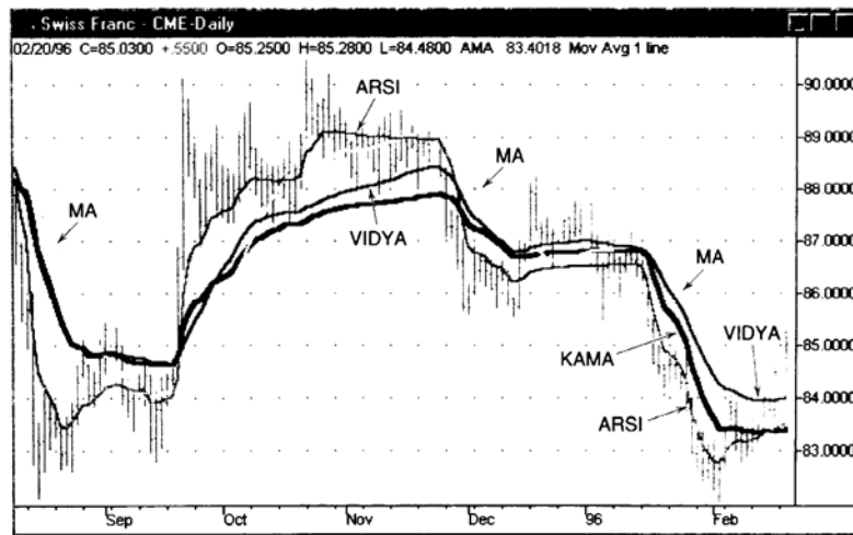
FIGURE17-1 Comparison of moving average, KAMA, VIDYA,AR2, and ARSI.
