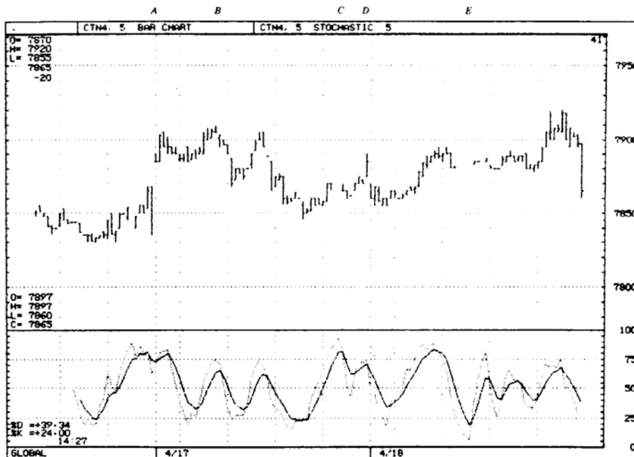
FIGURE 6-7 The stochastic. A 5-minute bar chart of July 1984 cotton futures (New York Cotton Exchange) as recorded by a Commodity Quote-GraphicsTQ-20120 satellite system. Cotton's 5period stochastic is plotted below the bar chart.
