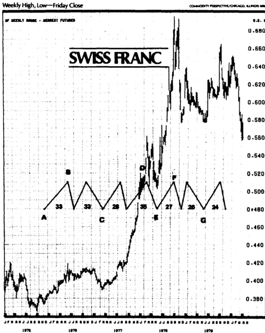
FIGURE 8-2 Cycles in Swiss franc futures.
