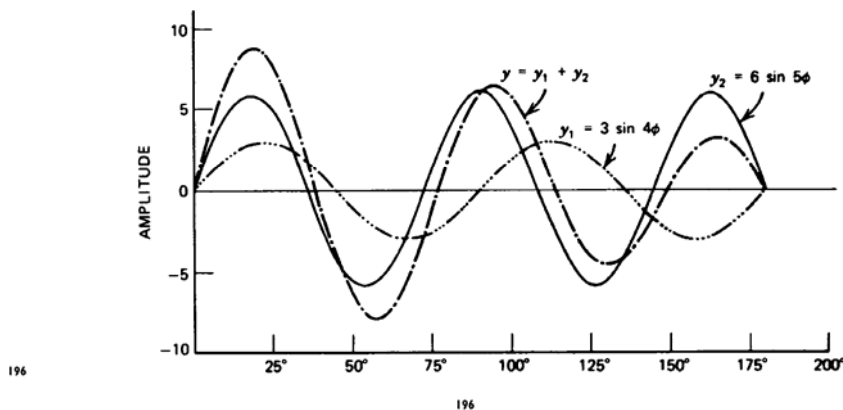
FIGURE 8-6 Compound sine wave.
