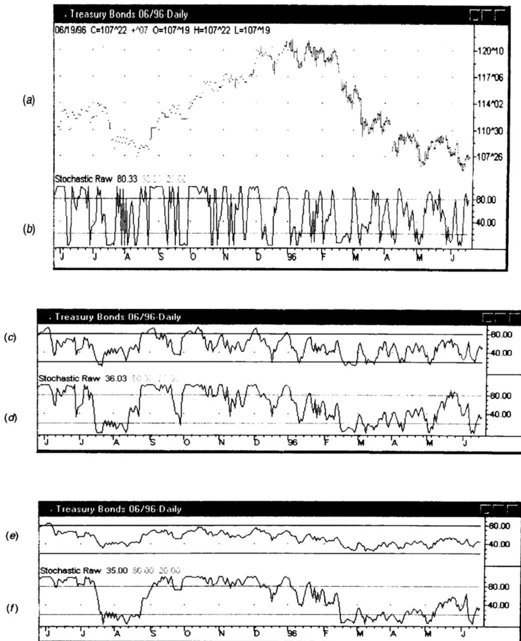
FIGURE 6-9 Comparison of RSI and stochastic. (Panel a) Treasury bond prices for the June 1996 delivery. (Panel b) The 5-day raw stochastic often reaches maximum and minimum Val. ues. (Panels c and d) Comparing the 5-day RSI with the 20-day stochastic. (Panels e and f) Comparing the 14-day RSI with the 40day stochastic.
