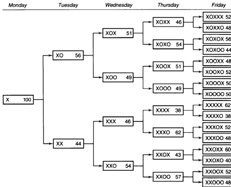
(b) S & P 500
