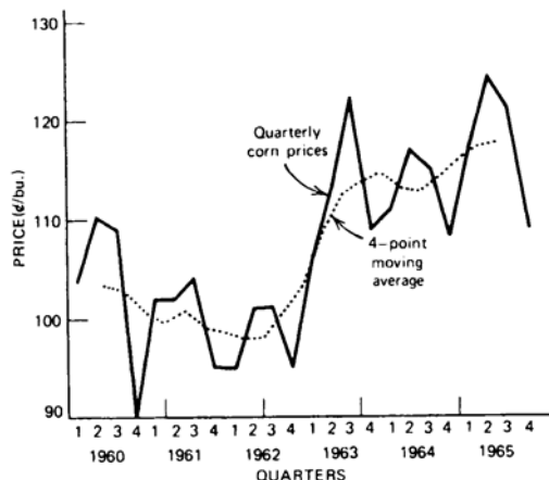
FIGURE 7-3 Detrending corn using a moving average with a yearly period.
